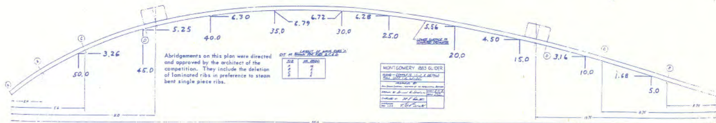
The airfoil section of the 1883 glider
